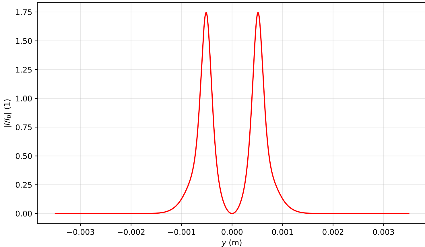
Intensity profile I(x=0, y, z=0.398)/I_0 , P_{in}=9.0P_{cr} , artificial time
